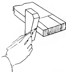
FIG. 259. LAYING OFF MORTISE FOR KEY OR WEDGE.
